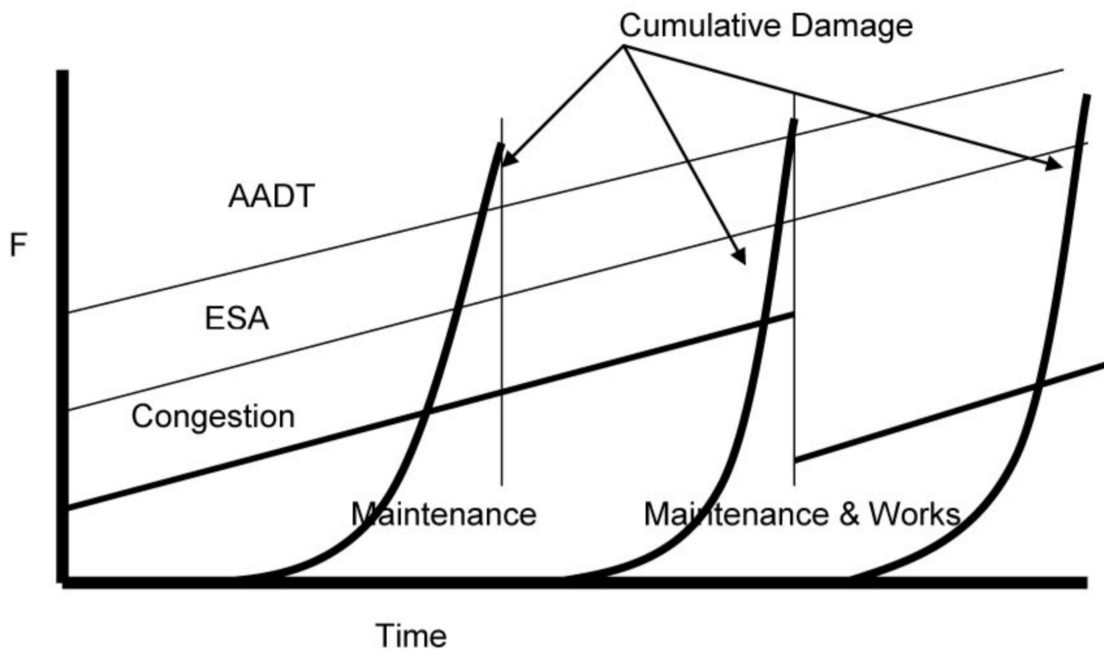
Figure 5: Cycle of Cumulative Damage for a Pavement
